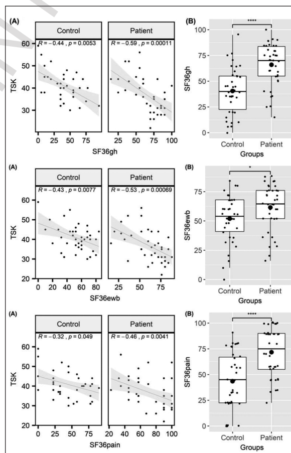
FIGURE 1: Analysis of the correlation between the Tampa Kinesiophobia Scale (TKS) and SF-36 emotional well-being and general health parameters in patient and control groups.
